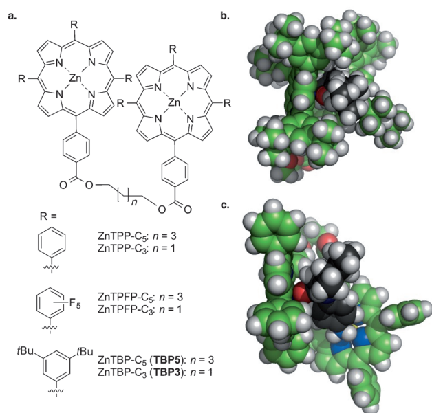
Figure 1. Bis(porphyrin) tweezers: a) Structures of porphyrin tweezer. b) TBP3 tweezer complex with 1 . c) TPP3 tweezer complex with 1 (MMFF, Spartan 14).
